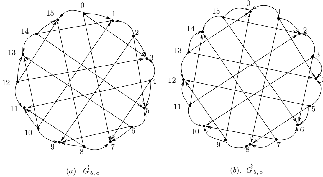
Fig. 4: Graphs \vec{G}_{5,e} and \vec{G}_{5,o} .
