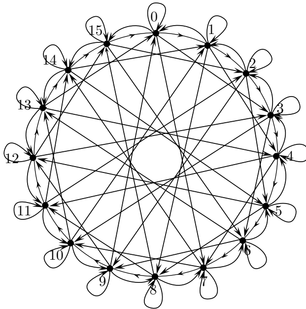
Fig. 2: The Circulant digraph \vec{G}'_5 = \overrightarrow{\text{Circ}}(16, \{0, 1, 3, 7, 15\}).
