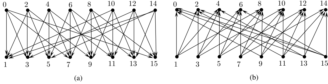
Fig. 5: Redrawings of \vec{G}_{5,e} and \vec{G}_{5,o} , in Figure 4, in the “natural” bipartite structure. For example the edges of distance 7 in \vec{G}_{5,e} are edges of jump 3 from X to Y , where X = \{0, 2, 4, \dots, 14\} and Y = \{1, 3, 5, \dots, 15\} , in the bipartite structure. Actually, an edge of distance 2^\ell - 1 in \vec{G}_{k,e} becomes an edge of jump 2^{\ell-1} - 1 , from X to Y , in the bipartite structure. As the graphs of Figures 4(a) and 4(b) are isomorphic, the graphs in Figures 5(a) and 5(b) are isomorphic (the isomorphism is obtained by mapping the vertex i in Figure 5(a) to i + 1 \pmod{2^{k-1}} of Figure 5(b)).
