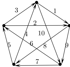
(c). An aneulerian tour in \vec{K}_5 is described by the arc sequence 1, 2, 3, ..., 10, taken in that order.
