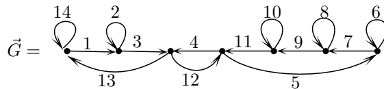
(d) An aneulerian tour in \vec{G} with directed loops at some of its vertices is given by the arc sequence 1, 2, ..., 13, 14, where the directed loops are traversed in the forward or backward direction in order to have an aneulerian tour in \vec{G} .
