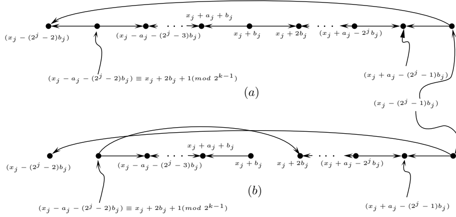
Fig. 6: Figure 6(a) shows the cycle \vec{C}_{j,o}^{2^{j-1}} as in (4) above and Figure 6(b) shows the reconstructed anti-directed path \vec{H}_{j,o}^{2^{j-1}} with origin x_j - (2^j - 2)b_j and terminus x_j + b_j .
