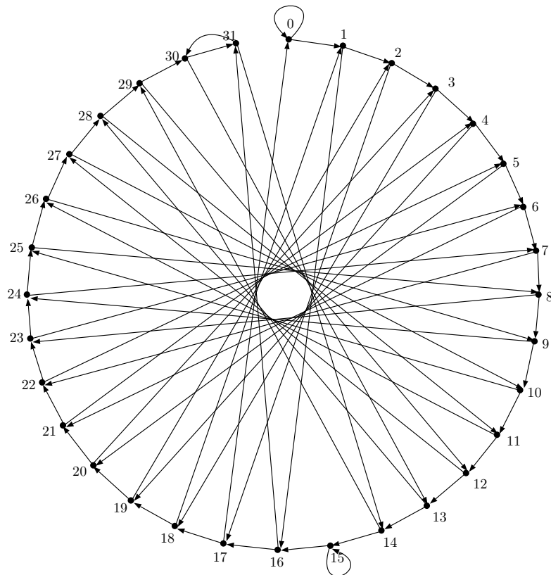
Fig. 9: A spanning 2-diregular biculerian subdigraph \vec{H}_1 of \vec{C}_6' .
