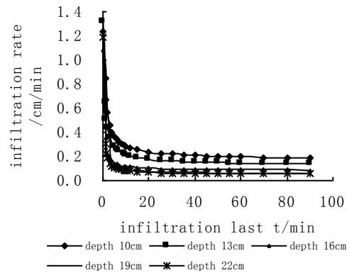
Figure 4-b Changing curves of the infiltration rate at given time with different depths
