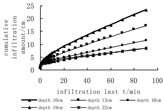
Figure 4-a Changing curves of the cumulative infiltration amount at given time with different depths
