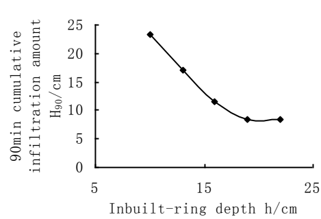
Fig.6 Changing curve of the infiltration rate at 90 minutes with inbuilt-ring depths
