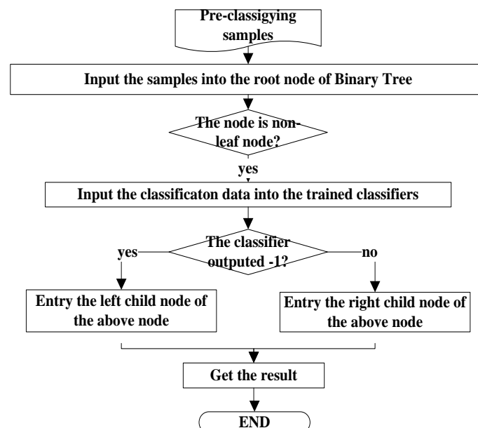
Fig.4. Classification Algorithm
