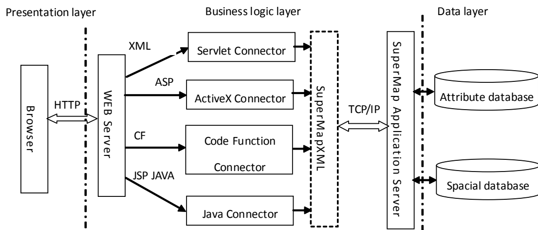
Fig.1 System architecture
