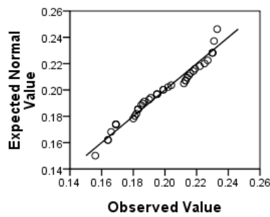
Fig.4 Normal Q-Q plot of June 4th
