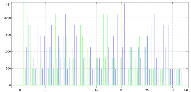
Fig. 13. Amount of data sent according to the elapsed time. In green are the results (in bytes) for the front vehicle and in blue for the back vehicle.
