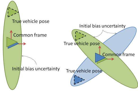
(a) The common frame is the one of the blue vehicle. Dashed triangles: true poses. Plain triangles: estimates. (b) The common frame is a new one. Dashed triangle: true pose. Plain triangle: estimate.
