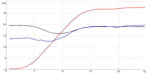
Fig. 14. Distance between both vehicles during the trajectory. In black is the true distance separating the vehicles. In red is the one computed from the SLAM results. In blue is the distance computed thanks to the decentralized localizations. The closer to the black curve, the better the results are.
