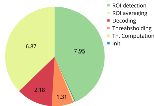
Figure 13: Steps duration repartition of the optimized algorithm
