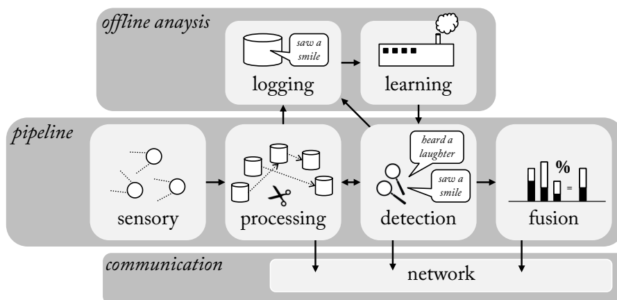
Fig. 1. Scheme of the laughter recognition component implemented with the Social Signal Interpretation (SSI) framework. Its central part consists of a recognition pipeline that processes the raw sensory input in real-time. If an interesting event is detected it is classified and fused with previous events and those of other modalities. The final decision can be shared through the network with external components.
