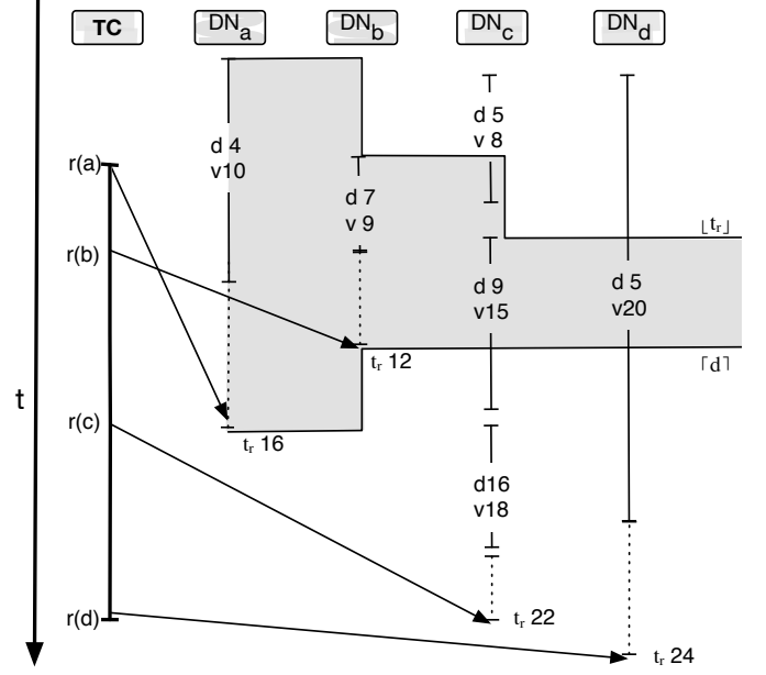
A TC builds a CCS by reading elements a, b, c and d from four different DNs . d , v and t_r represent an object's dependency, version and read timestamp, respectively.
