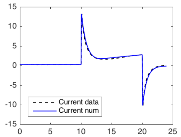
(b) Applied voltage amplitude: 460mV
