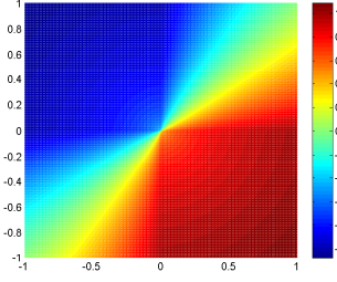
FIGURE 2. Map of \phi_{sing} when r_{\max} = 0.20 .
