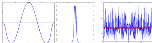
Figure 5: (Left): Inharmonic sinus (windowed by a smooth kernel to ensure continuous-derivable wrapping) and its Fourier modulus. (Right): PSD of a realization of white noise by points distribution and Bernoulli’s weights. Red: average of 100 realizations converges towards flat PSD.
