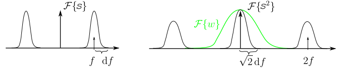
Figure 6: Spectrum of a bi-lobe noise (left) and of its square (right). The windowed second moment of the signal corresponds to the filtering of the latter by \mathcal{F}(w) (in green): it results in a LF lobe in Fourier, thus corresponding to LF contrast variations in image space.
