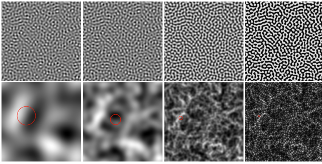
Figure 7: top: Blue noise normalized using different stationarity scales L . bottom: corresponding normalization field, i.e., variance filtered at the target window size (figured in red). NB: [min, max] is remapped to [0, 1] . The lower the frequency, the lower the amplitude of variations. On the third column the stationarity scale is the same as the wavelength of waves: each wave saturates the dynamics. On the fourth column the window scale is just a few pixels: the texture is forced to produce regions of min vs max value, with a sudden transition width equal to the stationarity scale.
