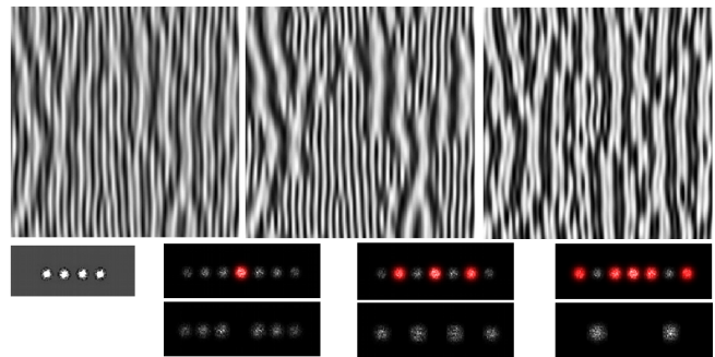
Figure 15: Same as Fig. 14 with aligned quadri-lobes.
