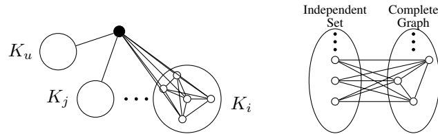
Fig. 2: Examples of graphs with unbounded neighborhood diversity and bounded twin-cover (left), and vice-versa (right). The left graph consists of a set of independent and disjoint cliques, all adjacent to a single vertex. The right graph is a complete bipartite graph where one side of the bipartition is a clique and the other is an independent set.
