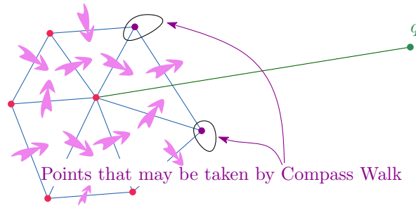
Figure 9: For the proof of Corollary 3
