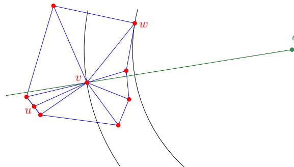
Figure 10: Greedy walk is not a visibility walk
