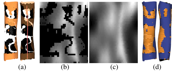
Figure 14: (a) Curve-skeleton prior for reconstruction from an incomplete point cloud [?]. (b) The cylindrically parametrized point-to-skeleton distance where missing data is marked by black pixels. (c) In parameterization space, the distance is inpainted into regions of missing data by minimizing a thin-plate energy. (d) The inpainting and the inverse parameterization allows the insertion of additional samples to complete the geometry.
