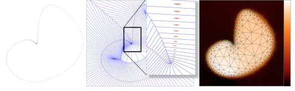
Figure 9: The reconstruction of an unoriented point cloud (left) is achieved by seeking for an indicator function \chi (right) whose gradients \nabla \chi match the anisotropy of the given covariance matrices (middle, shown as pink ellipsoids). These tensor constraints can be estimated from the second order moments of the Voronoi diagram of P (middle) [?].
