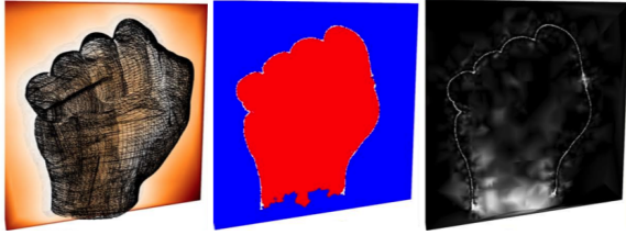
Figure 13: The approach of [?] first computes a robust unsigned distance function (left), and constructs an interior/exterior labeling (middle), and associated confidence (right) of the labeling. Note that low confidence is associated with regions of missing data, such as the bottom of the scan.
