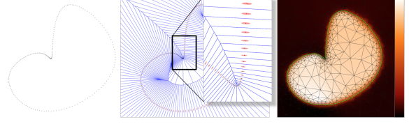
Figure 9: The reconstruction of an unoriented point cloud (left) is achieved by seeking for an indicator function \chi (right) whose gradients \nabla\chi match the anisotropy of the given covariance matrices (middle, shown as pink ellipsoids). These tensor constraints can be estimated from the second order moments of the Voronoi diagram of P (middle) [?].
