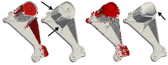
Figure 3: The impact of incorrect normal orientation. On the left we show the result of normal orientation via [?], where red splats indicate incorrect orientation. The results of running Poisson surface reconstruction [?] on this point cloud are shown in mid-left, where we indicate unwanted surface components due to the clustered normal flips. Similarly, on the right we show the orientation results of [?], and the corresponding results of [?].
