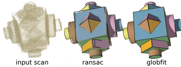
Figure 16: From a set of misaligned scans shown on the left, the primitives extracted via [?] (middle) retain the misalignment. Globfit [?] (right) is able to correct misalignment by enforcing consistent canonical relationships across primitives.
