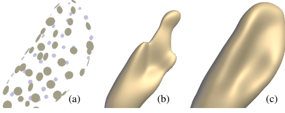
Figure 5: When sampling density is insufficient to resolve local curvature (a), the plane fitting operation employed by moving least squares [?] becomes highly unstable (b). APSS [?] addresses this by locally fitting spheres instead of planes. Using spheres tackles the aforementioned problem while remaining computationally inexpensive.
