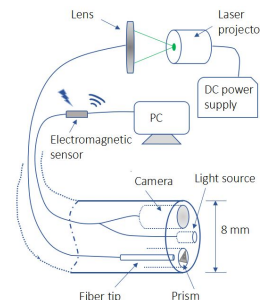
Figure 1. Configuration of the fiber-based endoscopic system.
