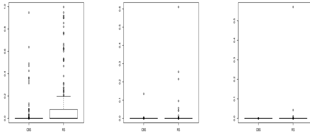
Figure 4: The boxplots of the p -values on the 200 replications for logit model with 20% causal variants, c = 1.3 , Q^* \approx 0.74 and 10%/90% of \theta(t_j) are negatives/positives (panels (a), (b), (c)). For logit model with 50% causal variants, c = 1.5 , Q^* \approx 0.78 and 20%/80% of \theta(t_j) are negatives/positives (panels (d), (e), (f)).
