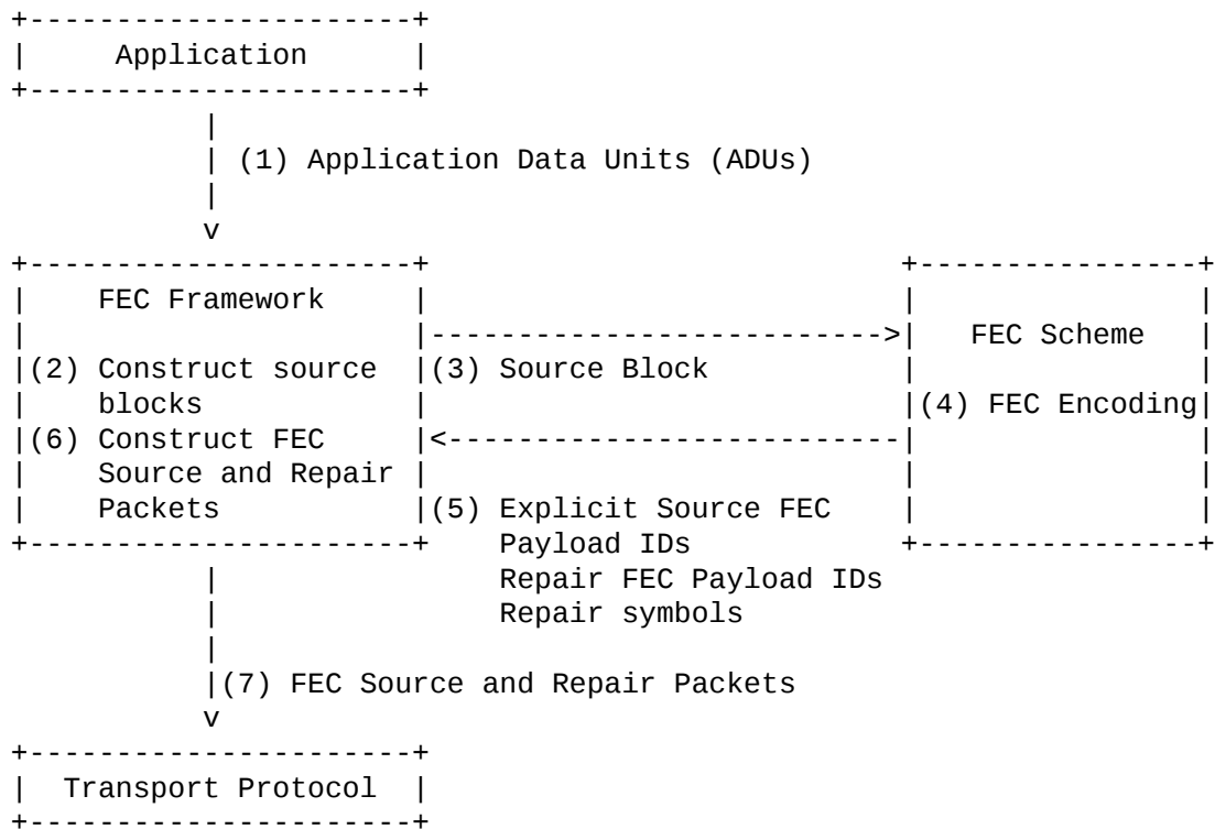
Figure 1: FECFRAME architecture at a sender.
