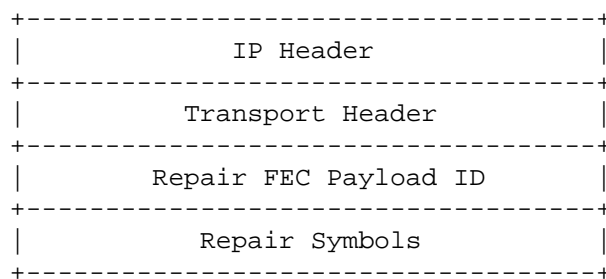
Figure 9: Packet Format for FEC Repair Packets
