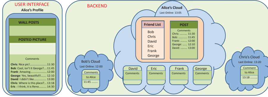
Fig. 11. Comment propagation
