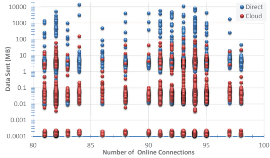
Fig. 7. Sender overhead for multimedia (log-scale)
