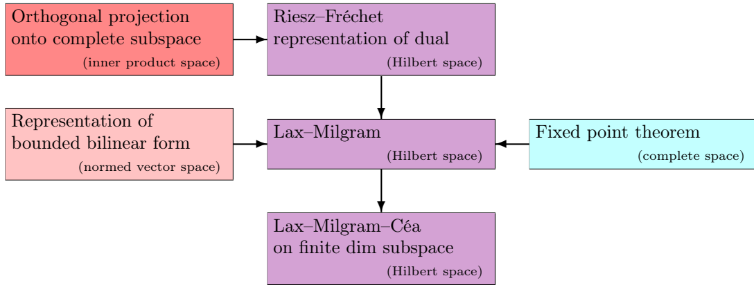
Figure 1: Hierarchy of results for a proof of the Lax–Milgram theorem.
