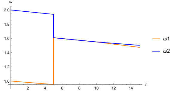
Figure 1: Simulation of the clutch model with resets. Mode change F \rightarrow T occurs at t = 5s and mode change T \rightarrow F occurs at t = 10s .
