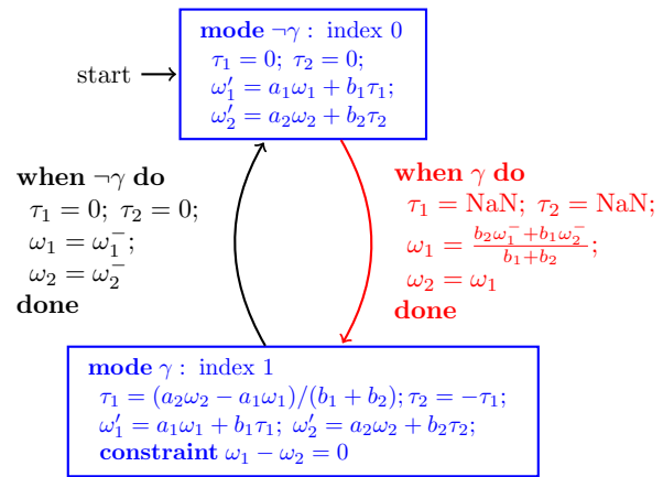
Figure 4: Standardization of the clutch's constructive semantics. Blocks have been standardized and then symbolically pivoted. x^- is the previous value of state variable x , which is the left limit of x when exiting a mode. Continuous-time dynamics are colored blue; non-impulsive (resp. impulsive) state-jumps are colored black (resp. red). The dynamics in mode \neg\gamma is defined by an ODE system, while in mode \gamma , it is defined by an over-determined index-1 DAE system consisting of an ODE system coupled to an algebraic constraint. In the transition from mode \neg\gamma to mode \gamma , variables \tau_1 and \tau_2 are impulsive, and their standardization is undefined. This explains why they are set to NaN (Not a Number).
