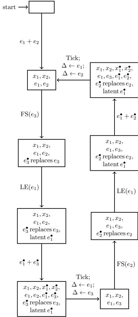
Figure 5: Constructive semantics of the overdetermined system. Notations are those of Fig. 3.
