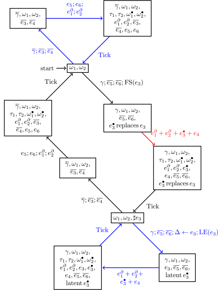
Figure 3: Constructive semantics of the Simple Clutch. Notations: For all statuses (shown in boxes), v (resp. \bar{v} ) means v = T (resp. v = F ), and not mentioning v means v = U . \#e means that e_f belongs to context \Delta . FS(\cdot) (resp. LE(\cdot) ; resp. \Delta \leftarrow \cdot ) refers to line 14, forward shift (resp. 16, latent equation; resp. 11, redundant equations) of Algorithm 5. Blue (resp. black) transitions belong to a continuous-time (resp. discrete-time) dynamics. The red transition is impulsive. A semicolon is the sequential composition of micro-steps, and the + sign denotes blocks of equations.
