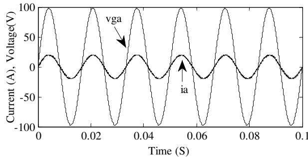
Fig. 3. DG current and grid voltage under interfacing impedance variation at the instant
