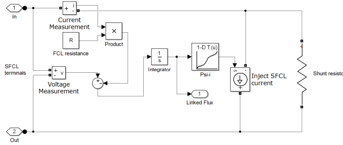
Fig. 4. Simulink model for the SFCL implementation.
