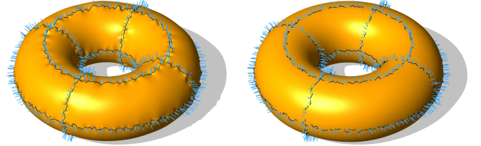
Figure 7: If the input data are noisy, soft constraints (right) produce better results than hard constraints (left) while still maintaining high overall shape fidelity. In this example, we artificially added 5% of noise to both positions and normals.
