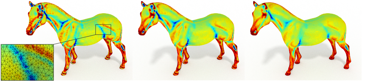
Figure 3: Mean curvature of the irregular horse mesh. (Left) the cotan formula [42] which is based solely on the mesh vertices, (middle & right) the 3-averaging formula (1), which additionally takes into account a normal at each vertex. For the middle image, the vertex normal is taken as the average of the face normals. In the rightmost example we smoothed the vertex normals before applying formula (1).
