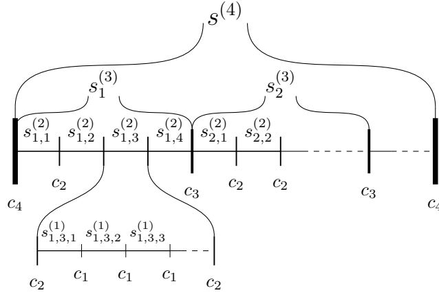
Figure 2: Example of a 4-level pattern. Here, we let c_\ell = C_1|C_2|\dots|C_\ell denote the succession of checkpoints from level 1 to level \ell .
