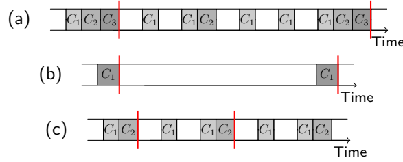
Figure 1: Checkpointing patterns (highlighted using red bars) with (a) k = 3 , (b) k = 1 , and (c) k = 2 levels.
