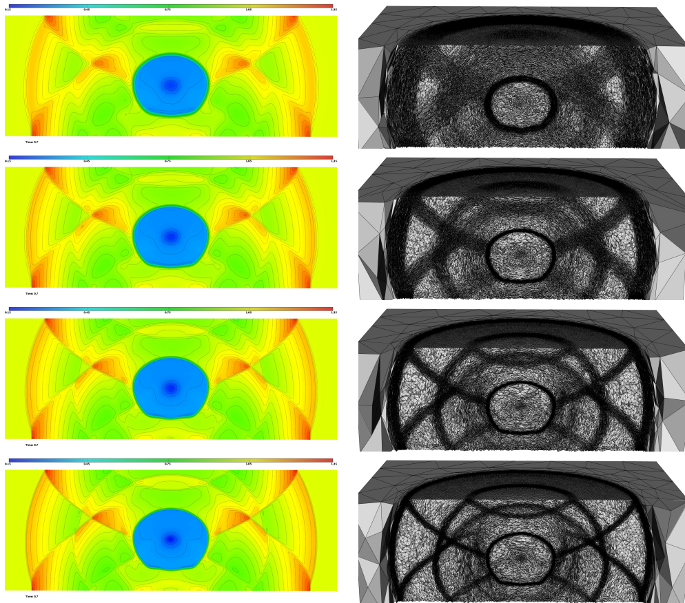
Figure 6: Spherical blast. Left, final solution at \alpha -dimensioned 0.7 for adaptive simulations with n_{adap} = 16 and \mathcal{N}_{avg} = \{40,000 ; 80,000 ; 160,000 ; 320,000\} (from top to bottom). It points out the solution - density field - accuracy improvement while increasing the average theoretical complexity of the adaptive simulation. Right, last sub-interval adapted meshes for adaptive simulations with \mathcal{N}_{avg} = 320,000 and n_{adap} = \{4 ; 8 ; 16 ; 32\} (from top to bottom).
