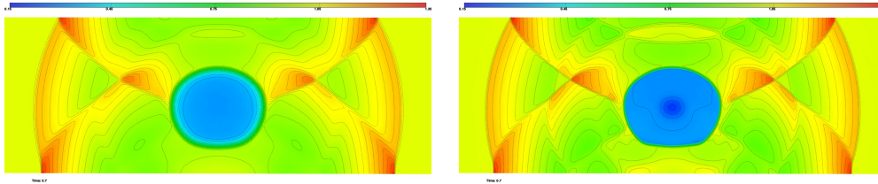
Figure 1: Final solution of a blast adaptive simulation (see Section 7.3) with 128 mesh adaptations. Left, using a classic \mathbb{P}_1 solution interpolation. Right, using the \mathbb{P}_1 -conservative solution interpolation.
