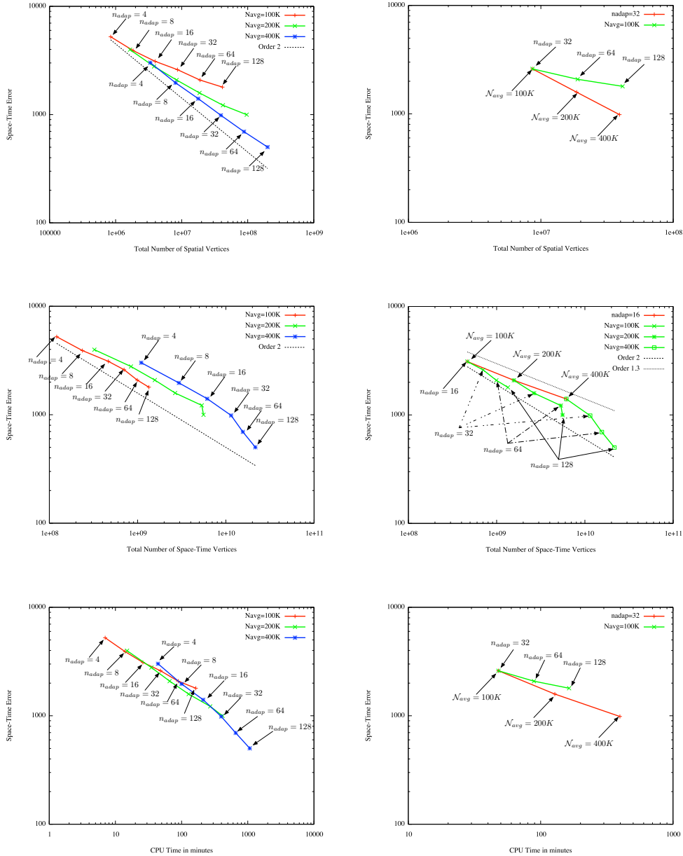
Figure 10: 3D blast in a city. Convergence curves of the space-time error with respect to the number of spatial vertices (top), the number of space-time vertices (middle), and the CPU time (bottom). Left, convergence curves for three prescribed average complexity with varying number of adapted meshes (sub-intervals). Right, convergence comparison between fixed average complexity with varying number of adapted meshes and fixed number of adapted meshes with varying average complexity.
