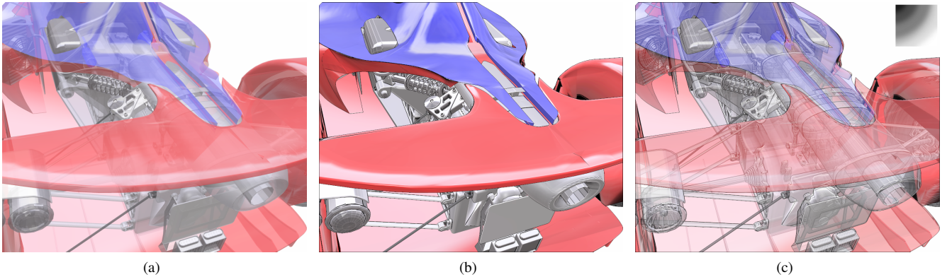
Figure 9: (a) OIT using a k -Buffer with a constant opacity value of 0.6 (50 FPS). (b) Mean Curvature Shading only. (c) Mean curvature transparency (20 FPS). The transfer function used is on the top-right corner. Model courtesy of dessindus.blogspot.fr . Times are obtained with a resolution of 1000 by 1000 pixels and 16 layers.
