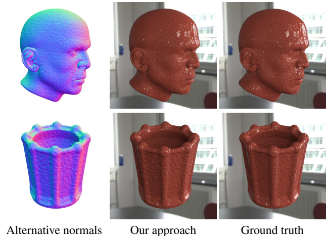
Figure 9: A Voronoi-based bump texture is mapped onto the red head and vase models in 3D, yielding an alternative normal buffer. Our approach is used to modify shading at the compositing stage in real-time, with a resulting appearance similar to re-rendering the object using the bump map (ground truth).
