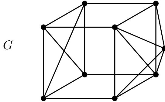
Fig. 3: \max_{v \in V(G)} \mathcal{H}_G(v) = \min_{v \in V(G)} \mathcal{H}_G(v) = 1 , sc(G) = -2 .
