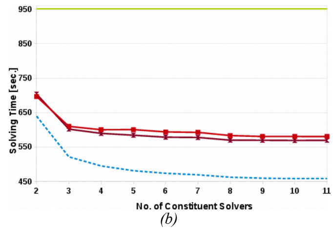
Figure 3: AST performance.
