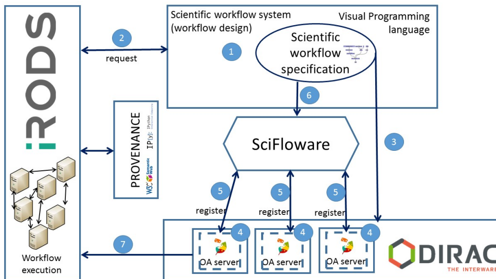
Figure 3: InfraPhenoGrid Architecture
