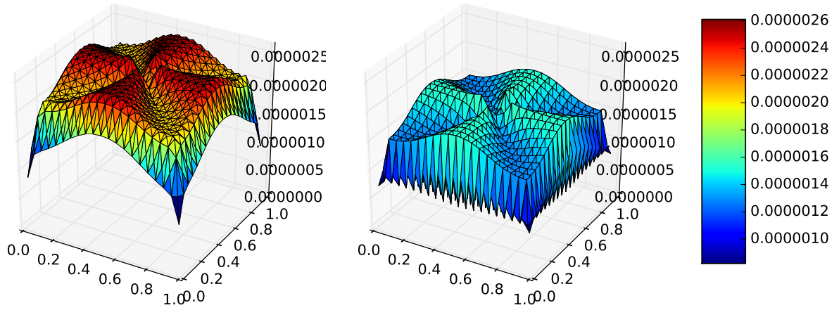
Figure 1: Functions \epsilon_{glob}^q (left) and \epsilon_{loc}^q (right) for the case Chaillou-Suri , p = 1.5 , \#\text{cells}=1600
