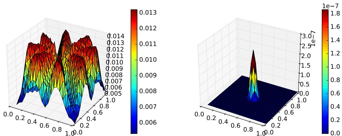
Figure 5: Functions \epsilon_{\text{glob}}^q (left) and \epsilon_{\text{en}}^p (right) for the case Chaillou-Suri , p = 10 , \#\text{cells}=1600
