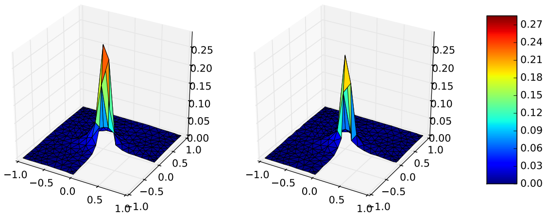
Figure 3: Functions \epsilon_{glob}^q (left) and \epsilon_{loc}^q (right) for the case Carstensen-Klose , p = 4 , \#\text{cells}=428
