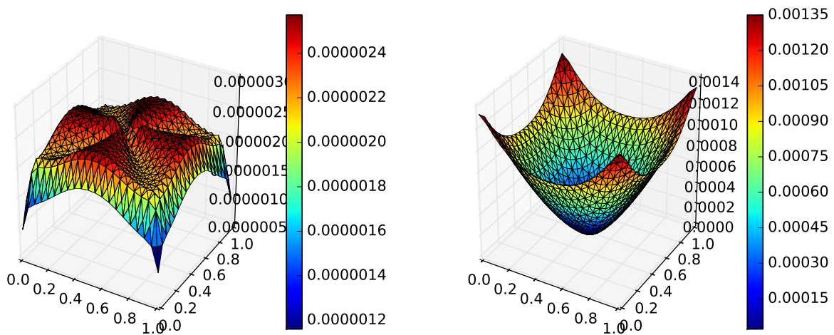
Figure 4: Functions \epsilon_{\text{glob}}^q (left) and \epsilon_{\text{en}}^p (right) for the case Chaillou-Suri , p = 1.5 , \#\text{cells}=1600
