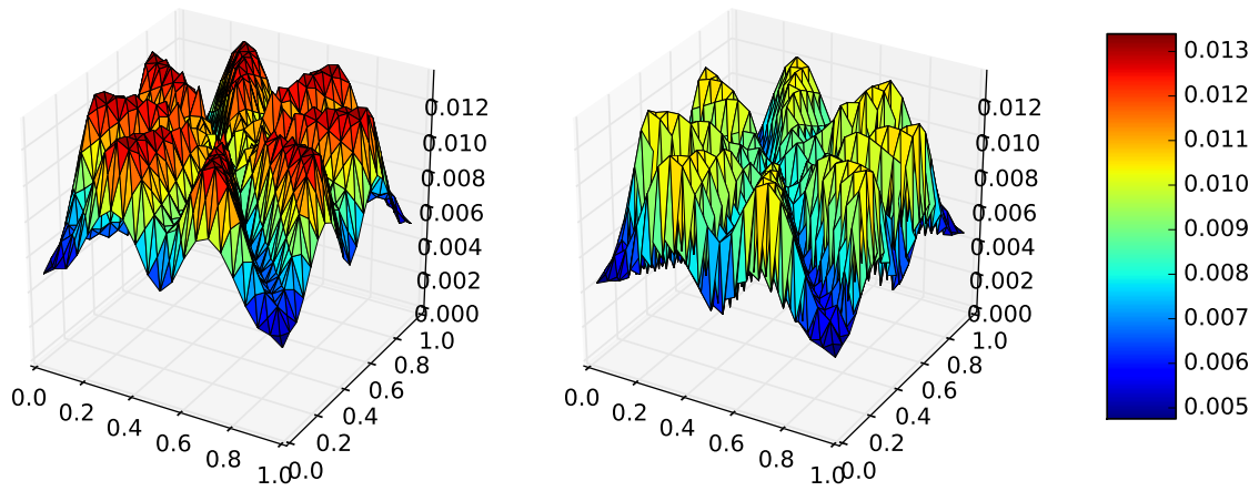
Figure 2: Functions \epsilon_{glob}^q (left) and \epsilon_{loc}^q (right) for the case Chaillou-Suri , p = 10 , \#\text{cells}=1600
