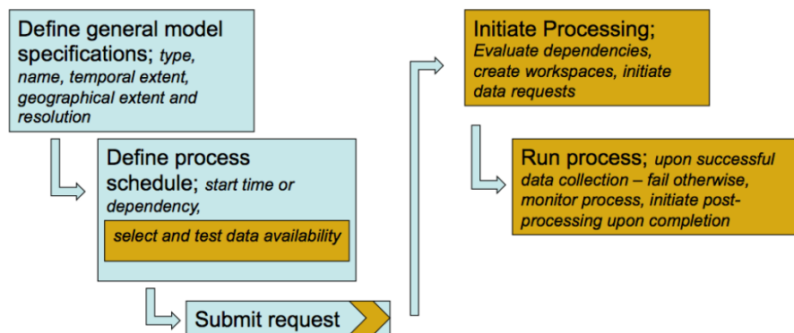
Fig. 3. The general workflow to initiate a TRIKE process, the background colours correspond to the location and correspondence of components in Figure 2.
