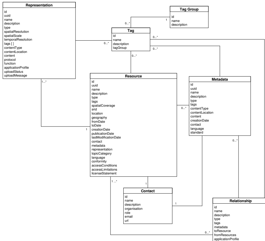
Fig. 3. Overview of relational model
