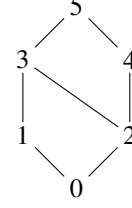
Figure 2. A Poset
