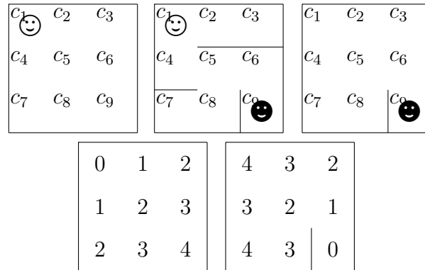
Figure 5: First step of simulation, ☺ represents Alice and ☹ represents Bob: G (at top center) and its internal representation for the agent \mathcal{G}_{\ominus}(1) (at top left) and \mathcal{G}_{\omin�}(1) (at top right) and the estimation by the agents of the distances d_{\ominus}(y, 1, E_{\ominus}) (at bottom left) and d_{\omin�}(y, 1, E_{\omin�}) (at bottom right).
