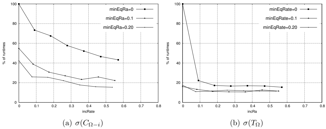
Figure 3: Percentage of runtimes where the agreements are fair.
