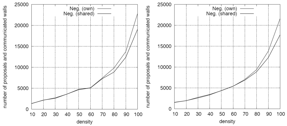
Figure 11: Number of proposals and communicated walls in simple mazes (at left) and in hard mazes (at right).
