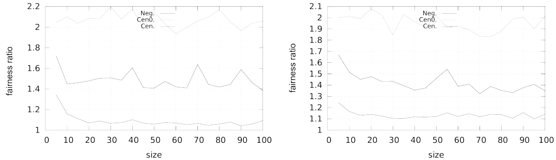
Figure 8: The fairness ratio (maximal number of steps / average number of steps) in some mazes. The simple mazes are generated with the pseudo-randomized version of Prim's algorithm (at left). The hard mazes are generated with the recursive backtracker algorithm (at right). The agents do not share their perception.
