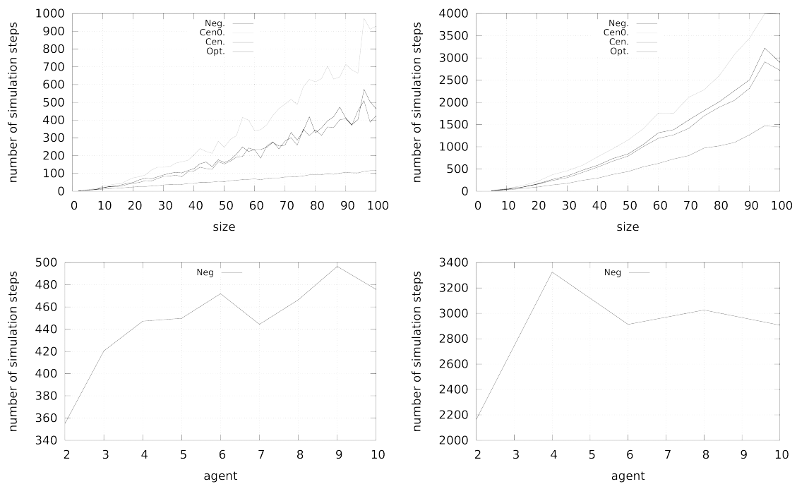
Figure 9: The number of simulation steps wrt the size of the maze (at top) and wrt the number of agents in 100 \times 100 mazes (at bottom) in some mazes. The mazes are simple (at left) and hard (at right). The agents share their perception.
