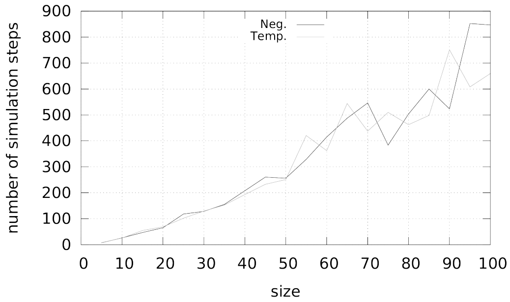
Figure 12: Number of simulation steps with the cooperative strategy (Neg) and the temporizing strategy (Temp).
