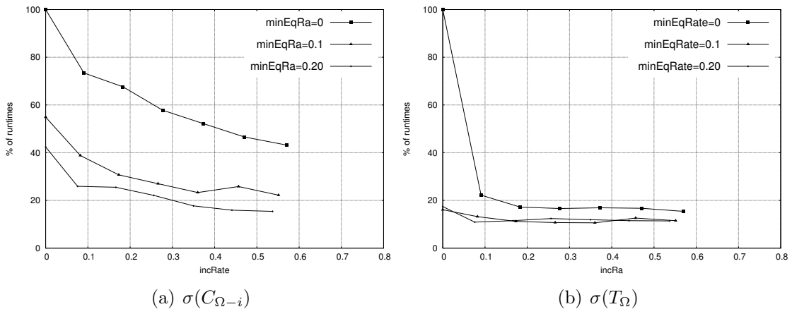
Figure 3: Percentage of runtimes where the agreements are fair.
