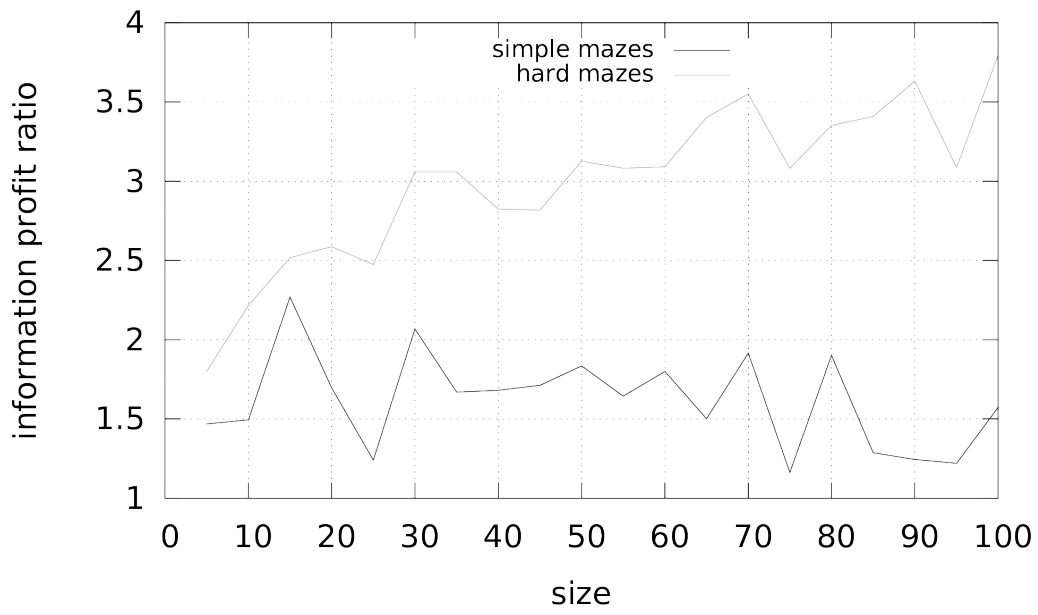
Figure 10: Information profit ratio for simple/hard mazes.
