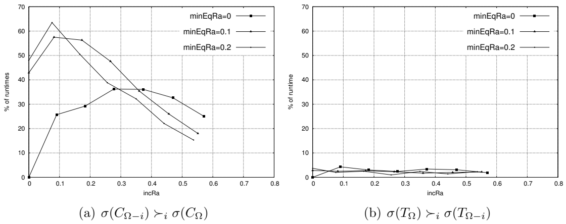
Figure 2: Percentage of runtimes where the temporizing strategy dominates the cooperative one.
