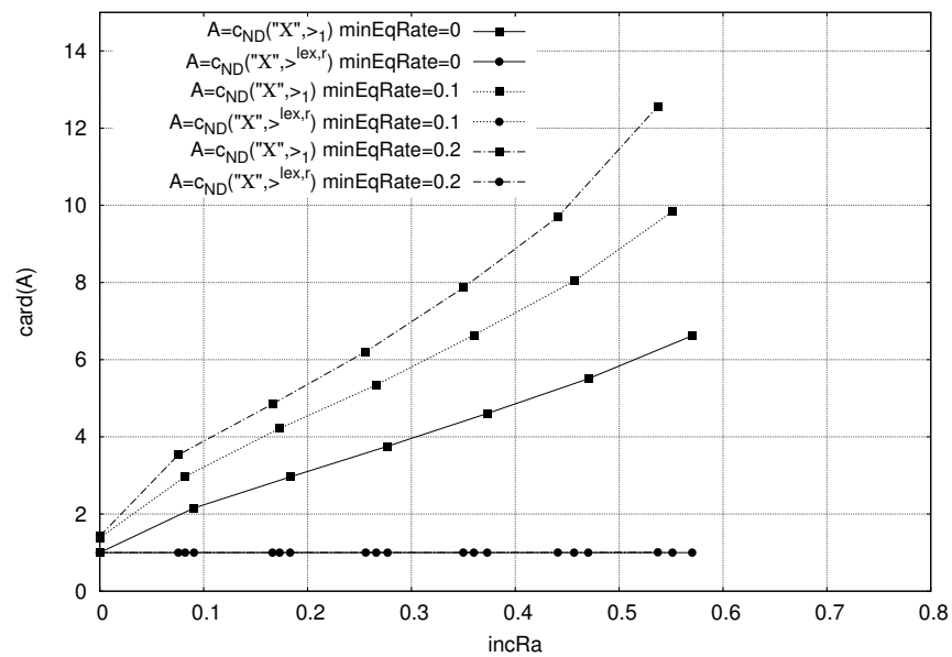
Figure 4: Cardinality of the non-dominated alternatives for the agent 1 and cardinality of the set of agreements when the all the agents cooperate ( \sigma(C_\Omega) ).
