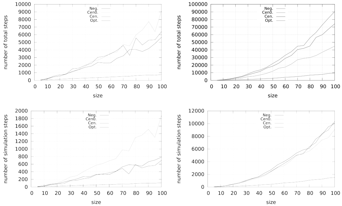
Figure 7: The number of total steps performed by the 10 agents (at top) and the number of simulation steps (at bottom) in some mazes. The simple mazes are generated with the pseudo-randomized version of Prim's algorithm (at left). The hard mazes are generated with the recursive backtracker algorithm (at right). The agents do not share their perception.
