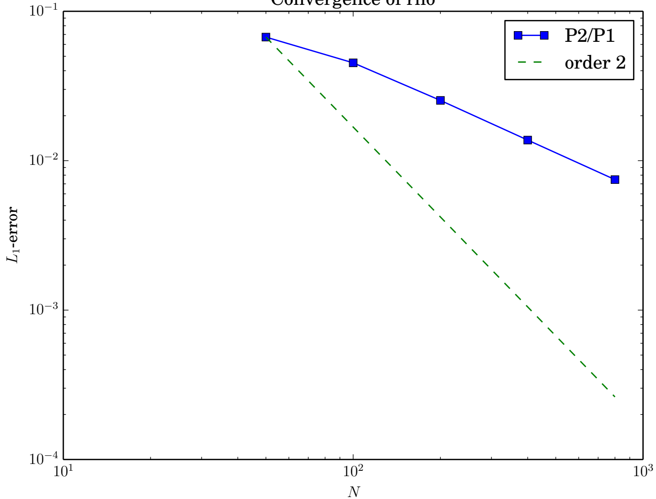
Convergence of rho
