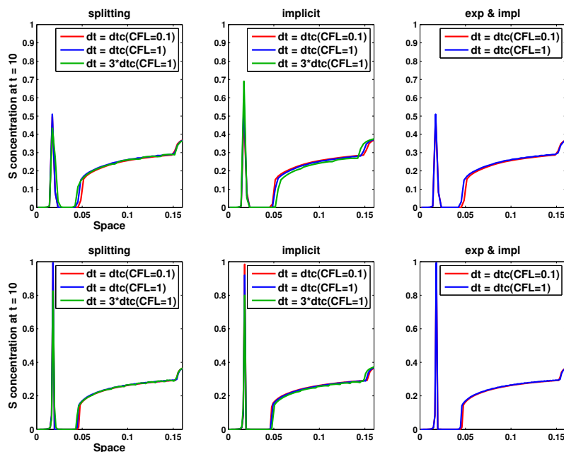
FIG. 6.7. Effect of the CFL condition on the concentrations in S (top figure 768 nodes, bottom figure 1536 nodes)
