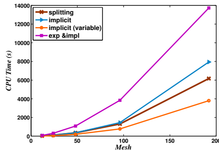
FIG. 6.8. CPU time required by the time discretization methods as the space mesh is refined
