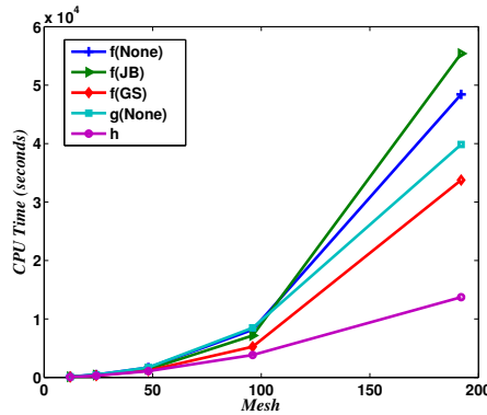
FIG. 6.10. CPU time as a function of the mesh size for the various solution methods
