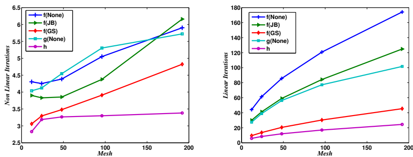
FIG. 6.9. Non-linear (left) and linear (right) iterations for different preconditioning strategies
