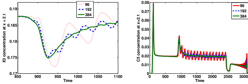
FIG. 6.4. Elution curves of X_3 (left) and C_5 (right) concentration, for various mesh resolutions
