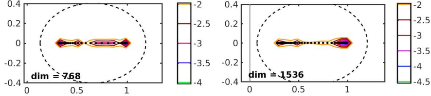
FIG. 6.11. Field of values (dashed line) and pseudo-spectra (color) for matrix J_h , with N_x = 768 and N_x = 1536
