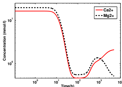
FIG. 6.12. Variation of \text{Ca}^{2+} and \text{Mg}^{2+} concentrations as function of time in the output of the domain
