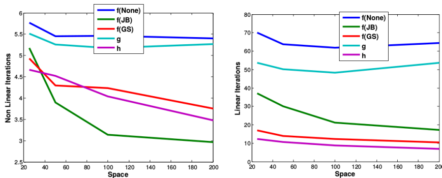
FIG. 6.13. Number of non-linear (left) and linear (right) iterations for ion exchange example
