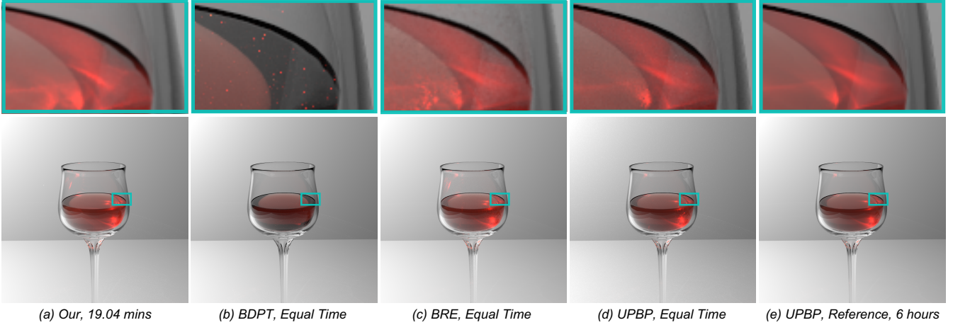
Figure 10: Material: wine, \alpha = \{0.1094, 0.0357, 0.0268\} , \ell = \{7.2992, 2.7472, 2.4207\} . For this material (low albedo, large mean free path), low order scattering effects dominate.
