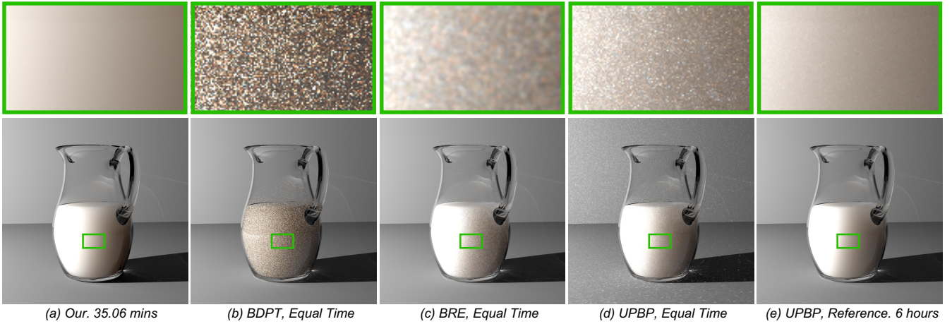
Figure 9: Material: milk, \alpha = \{0.9999, 0.9997, 0.9991\} , \ell = \{0.8422, 0.7521, 0.6848\} . For this material, with a very large albedo and a small mean free path, multiple scattering effects dominate.
