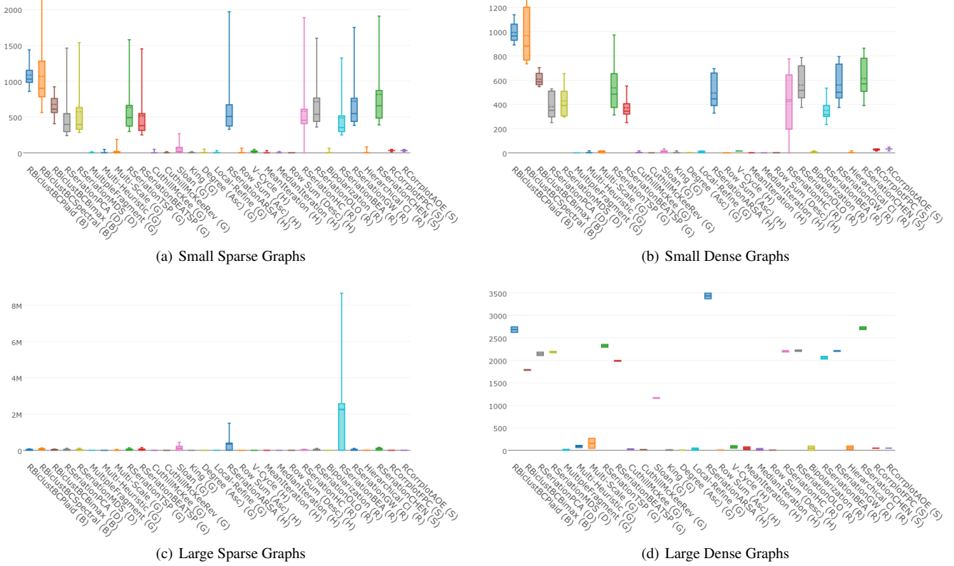
Figure 19: Calculation time (in msec) for each graph category (small/large versus sparse/dense).
