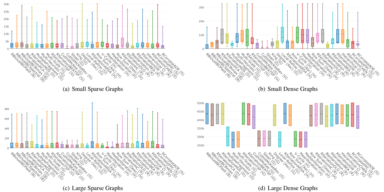
Figure 20: Linear arrangement Scores for each graph category (small/large versus sparse/dense).
