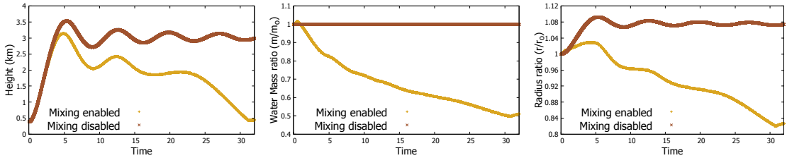
Figure 3: Attributes of a parcel varying with time in our simulation, with mixing enabled and disabled: ( left ) parcel position, ( mid ) parcel water mass ratio relative to its initial value, ( right ) parcel radius ratio relative to its initial value.
