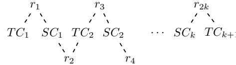
Figure 12: Weakly equivalent resources of G and their cliques.
