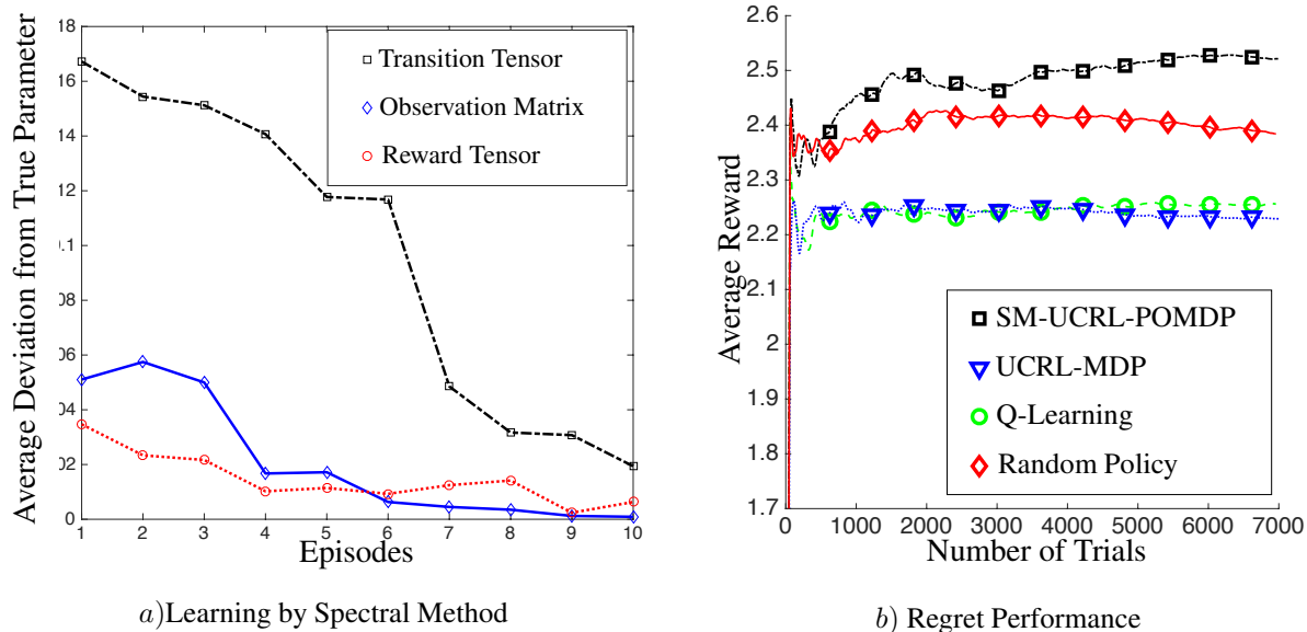
Figure 3: (a)Accuracy of estimated model parameter through tensor decomposition. See h Eqs. 11,10 and 12. (b)Comparison of SM-UCRL-POMDP is our method, UCRL-MDP which attempts to fit a MDP model under UCRL policy, \epsilon - greedy Q-Learning, and a Random Policy.
