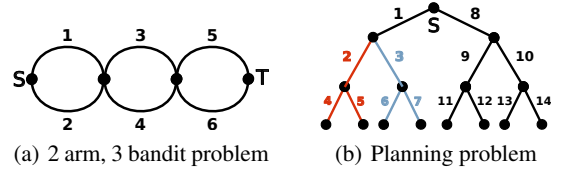
Figure 4: Examples of learning problems in which our algorithms perform well.
