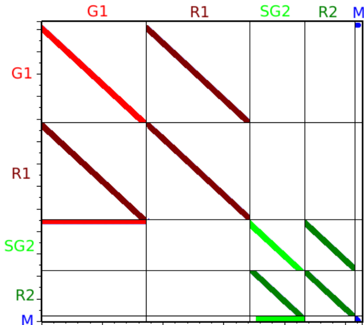
FIGURE 4. Pattern of the nonzero elements of the transition matrix of the discretised dynamics. Each block represents the transitions from one phase to the other. The block G_1/G_1 is a sub-diagonal matrix representing the fact that at each time step, the cells that have stayed in G_1 get older. The block R_1/R_1 is a diagonal matrix that represents cell proliferation arrest until cells go back to G_1 -phase .
